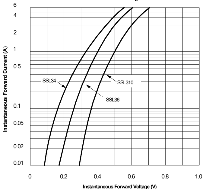
FIG.3: Forward Voltage
